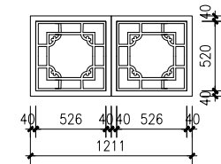
风窗大样1:25
