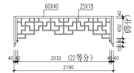
挂落大样1:25
